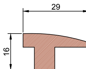
PERIMETER STRIP unfinished Oak 990mm or 3m length
