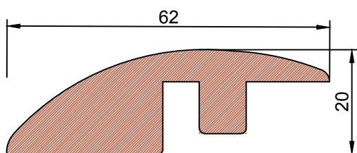
RAMP unfinished Oak 990mm or 3m length
