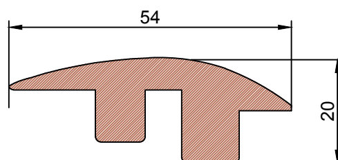
REDUCER unfinished Oak 990mm or 3m length
