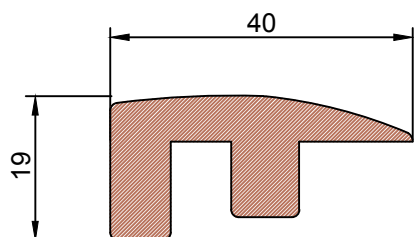
END PIECE unfinished Oak 990mm or 3m length
